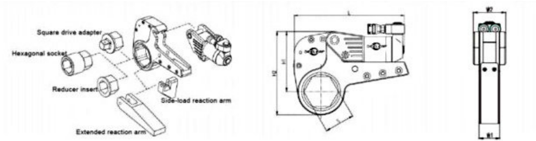
Hydraulic Bolting Tools - Hollow Hydraulic Wrench - Technical Parameters
