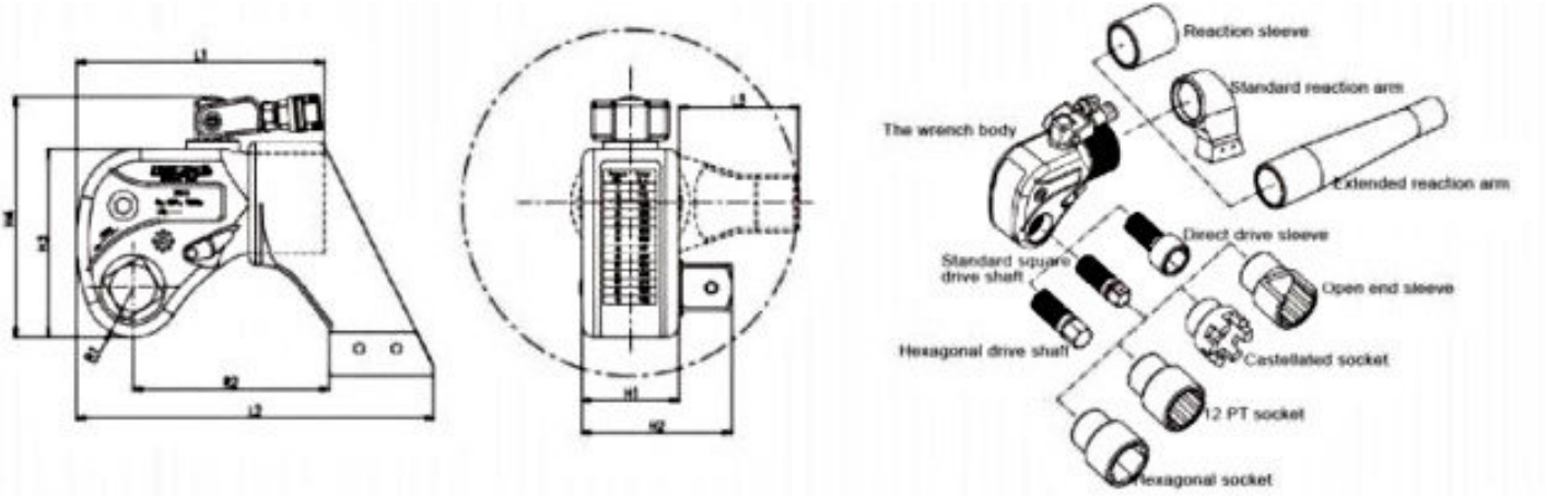
Hydraulic bolting tools - Driven type hydraulic torque wrench - Technical Parameters
